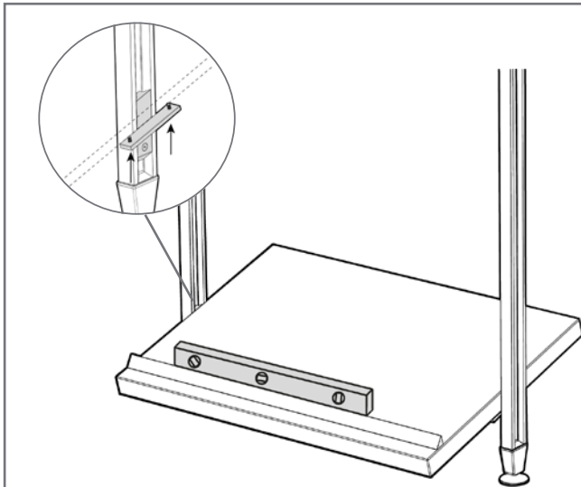
23 Position the shoe rack onto the brackets and level up. Once level secure the shoe rack into position by using the bolts supplied. (You will require a 4mm allen key.)
