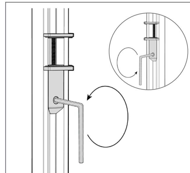
13 Position and lock both brackets onto the stanchions.
